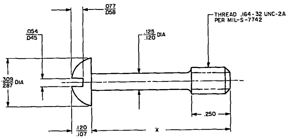
FIG 1. SLOTTED HEAD
