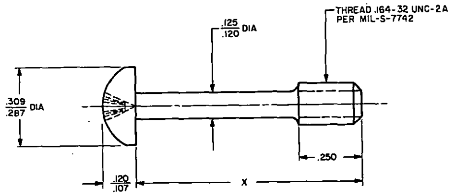
ⓑ FIG 2. CROSS-RECESSED HEAD
